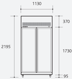
Integral/remote front elevation
