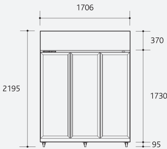
Integral front elevation
