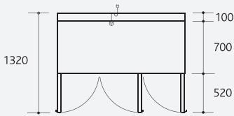
Integral top view
