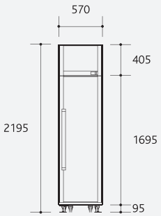
Integral front elevation
