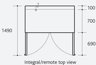
Integral/remote top view
