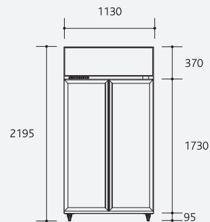
Integral/remote front elevation
