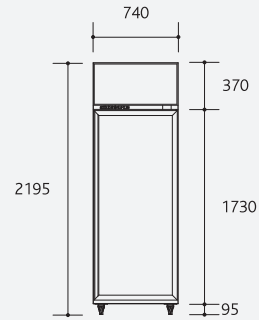
Integral/remote front elevation
