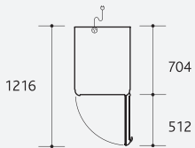
Integral top view
