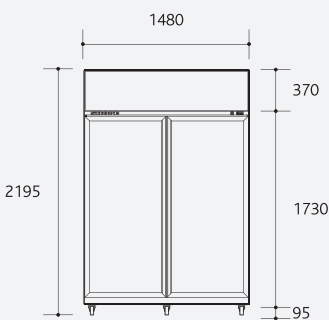
Integral/remote front elevation
